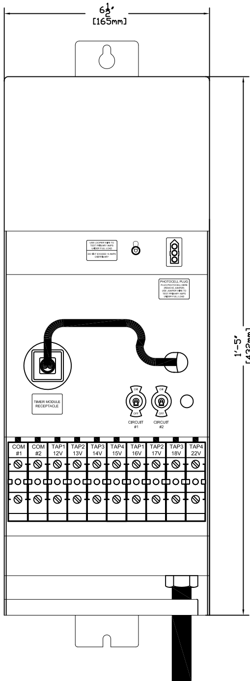
FRONT VIEW WITHOUT COVER
