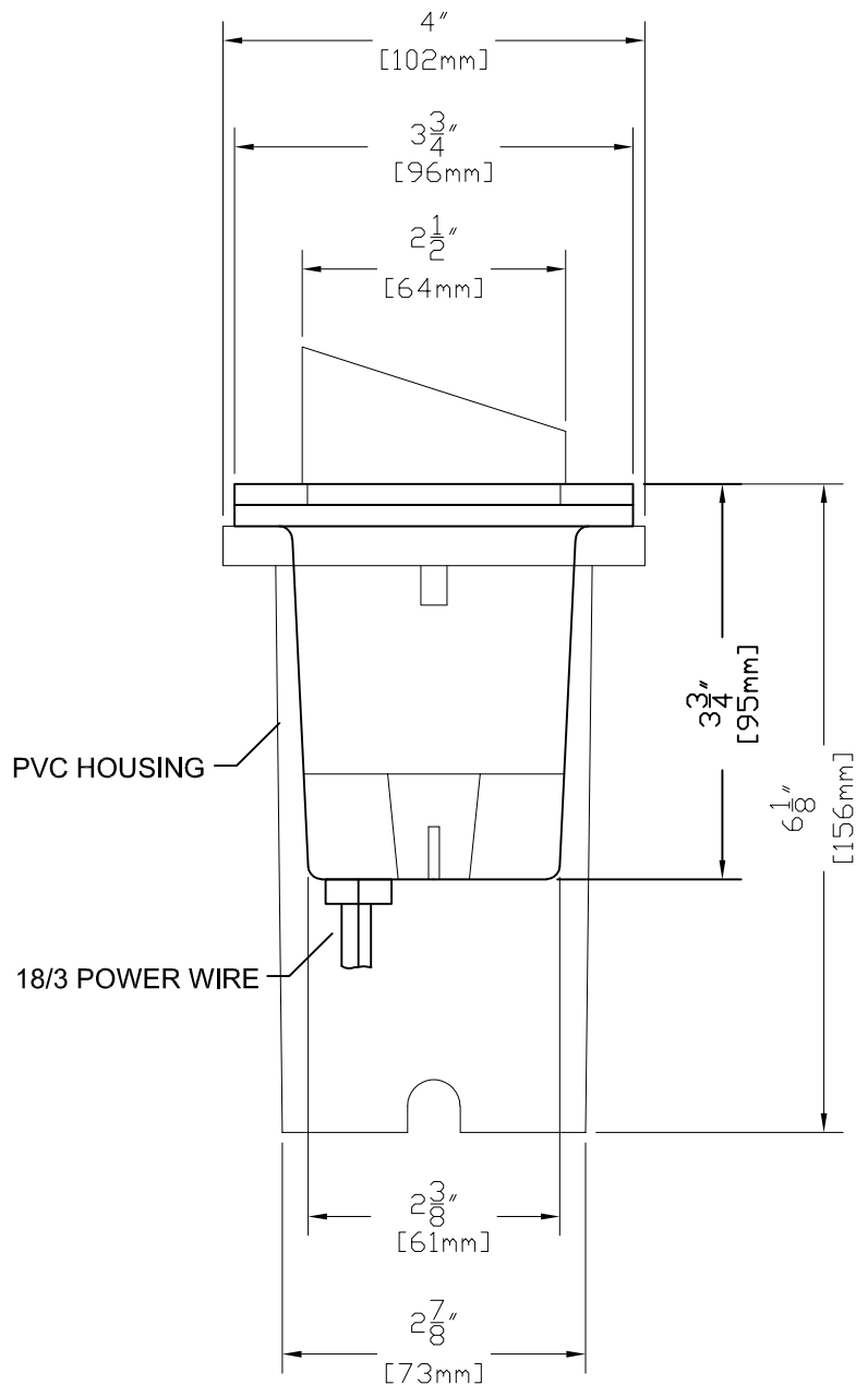
SIDE VIEW WITH DIMENSIONS
