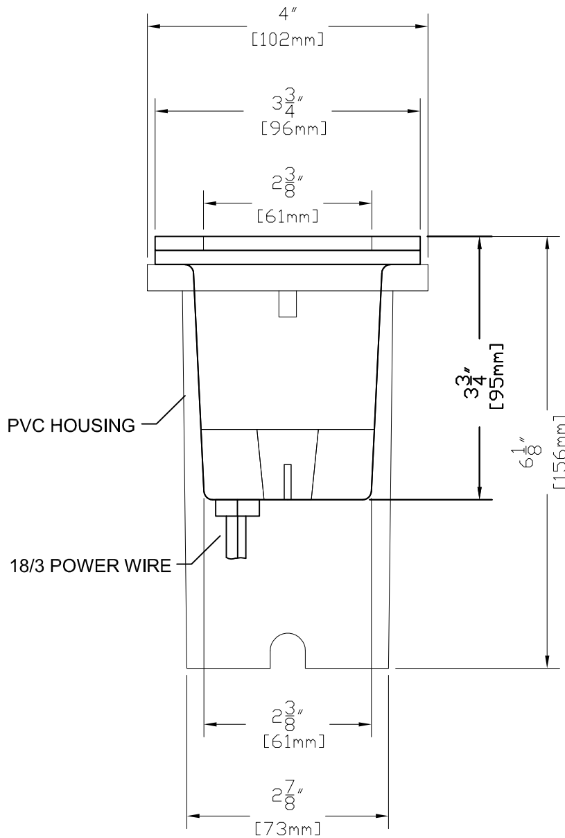
SIDE VIEW WITH DIMENSIONS
