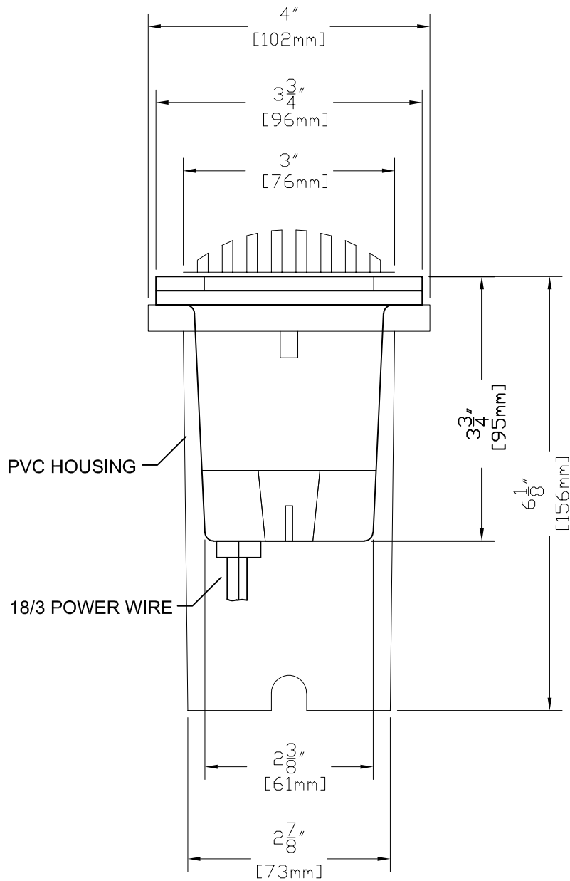
SIDE VIEW WITH DIMENSIONS
