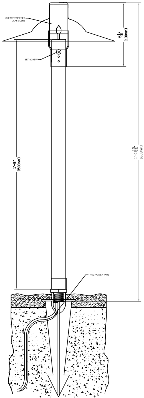
SIDE VIEW WITH DIMENSIONS
