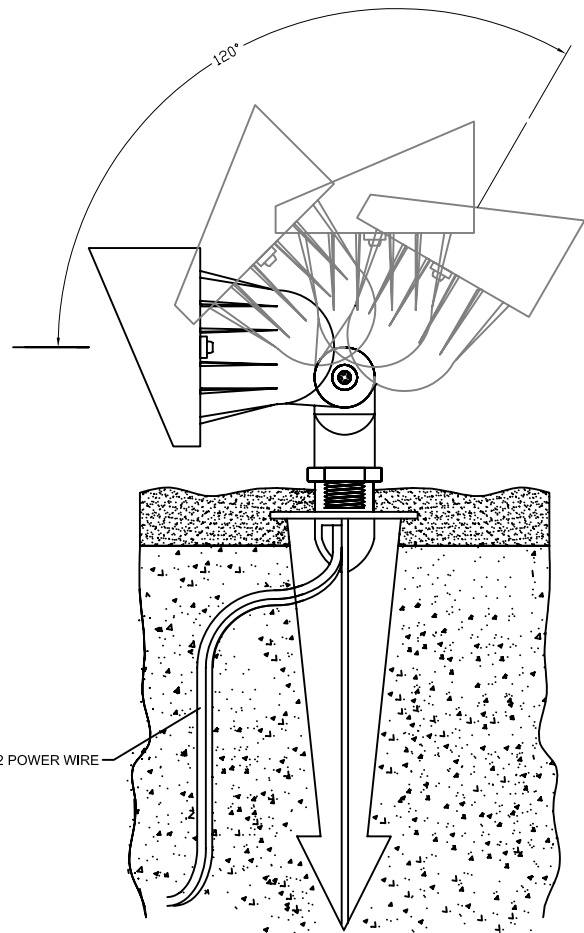
SIDE VIEW WITH ROTATION
