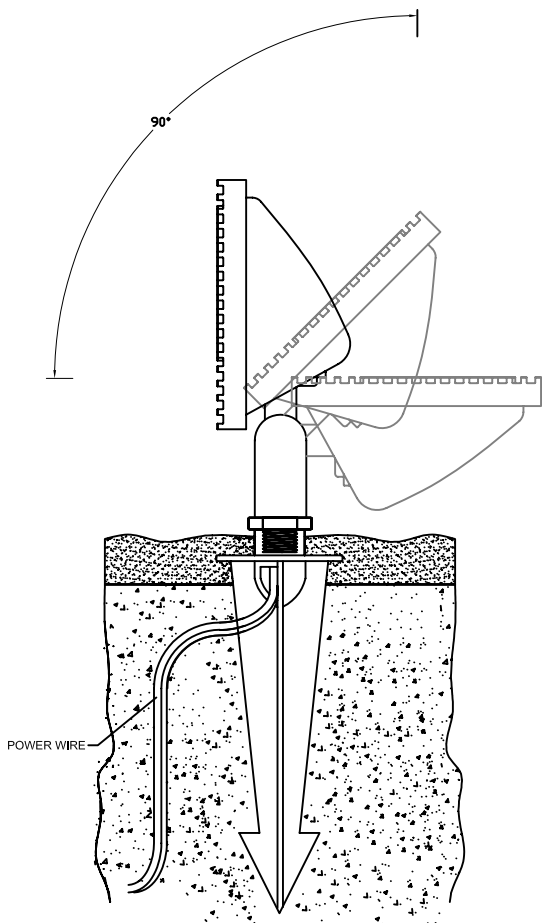
SIDE VIEW WITH ROTATION
