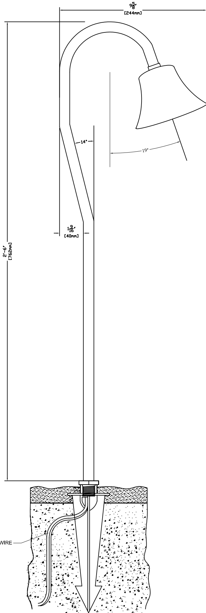
SIDE VIEW WITH DIMENSIONS
