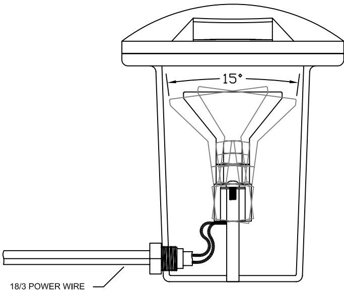
SIDE VIEW WITH ROTATION
