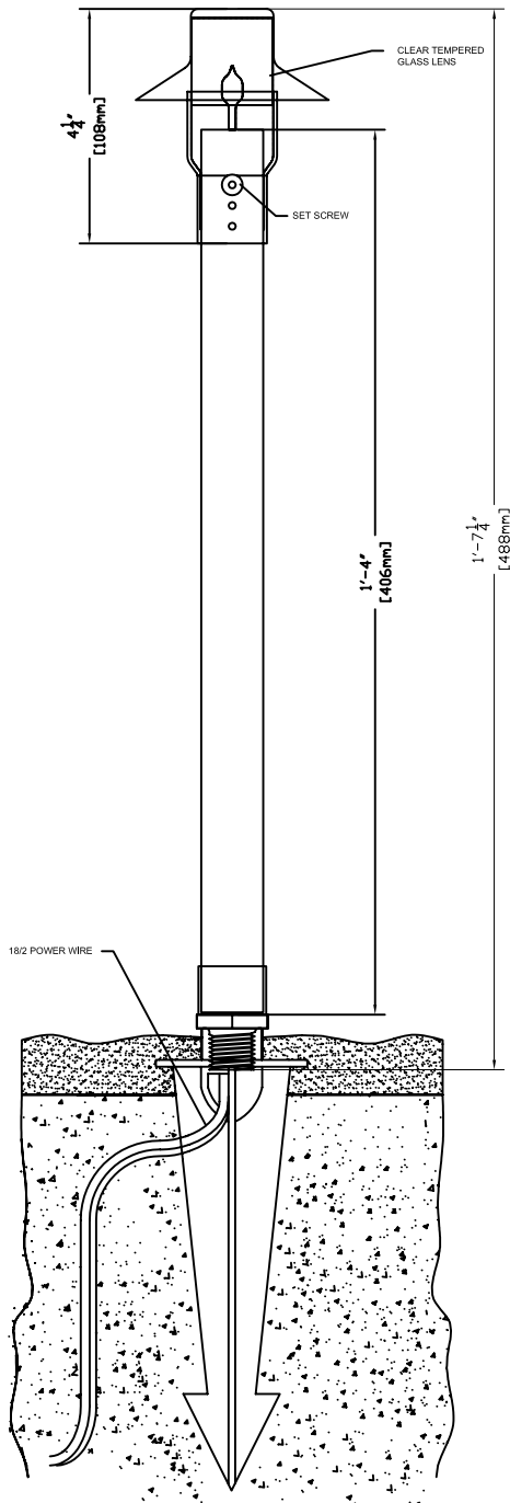
SIDE VIEW WITH DIMENSIONS
